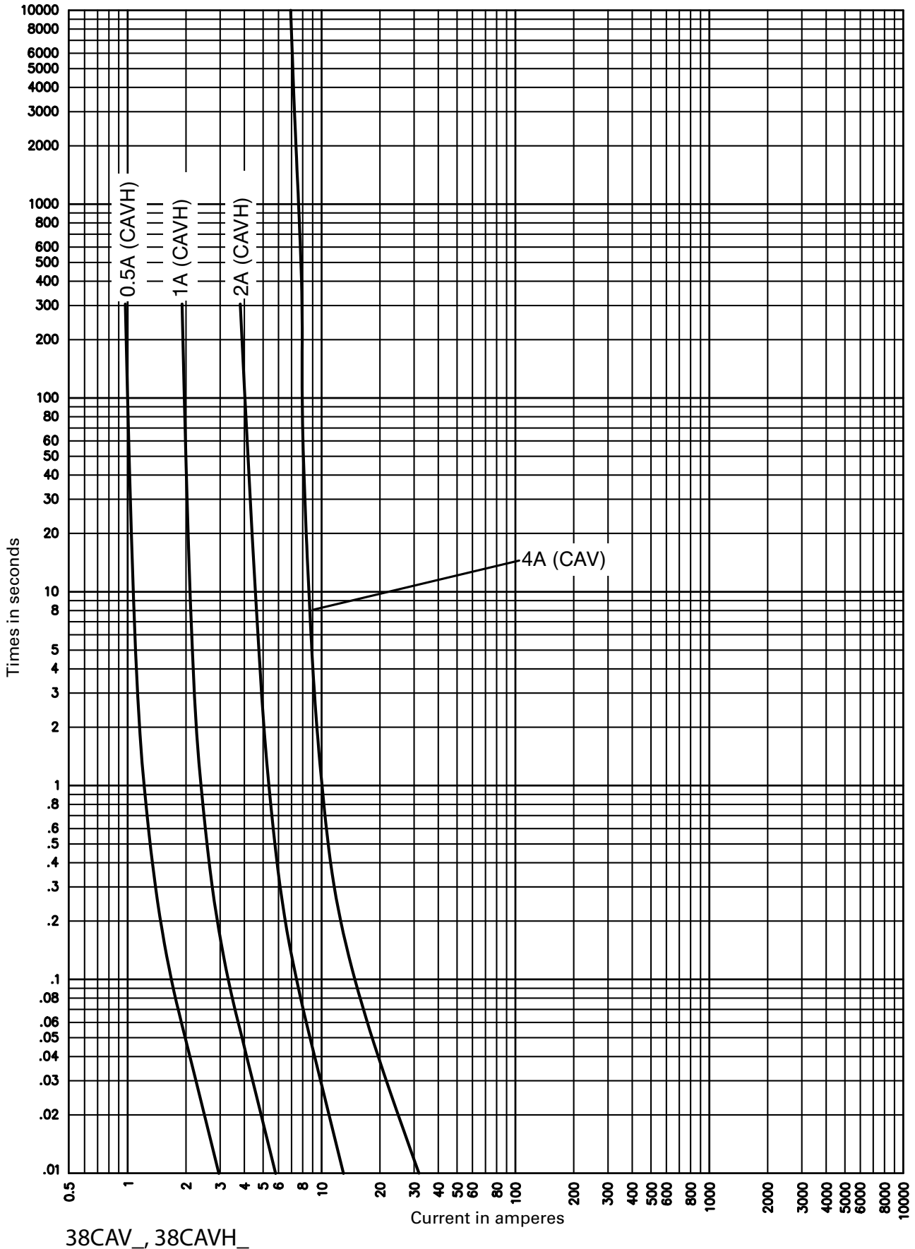
38kV time-current curves — minimum melting for 38CAV_ and 38CAVH
