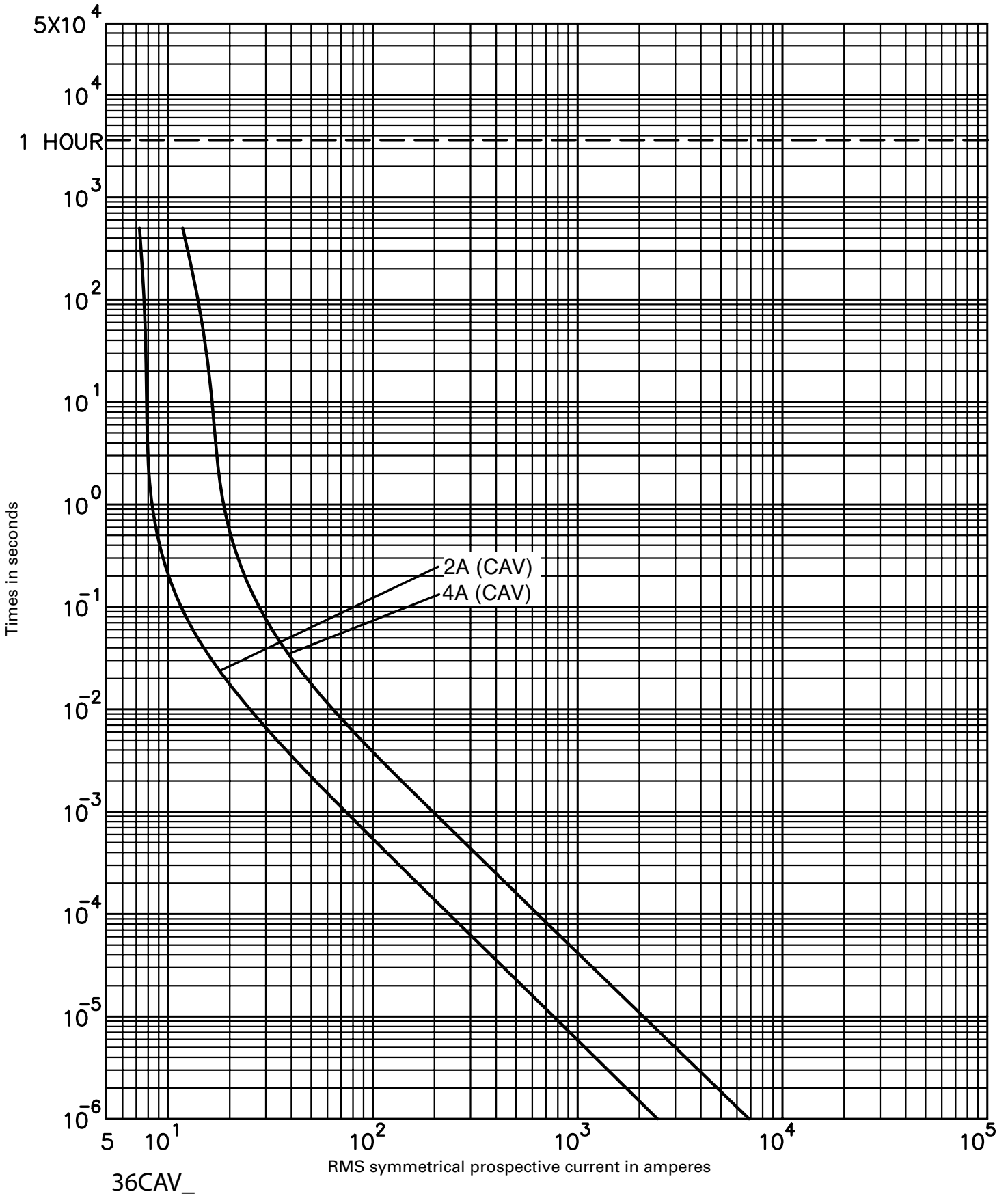
36kV Time-current curves — minimum melting for 36CAV_
