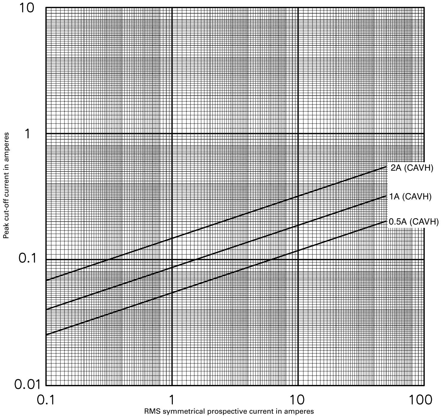
15.5kV peak let-through curves for 15.5CAVH_
