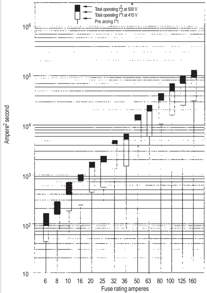
I^2t characteristics
