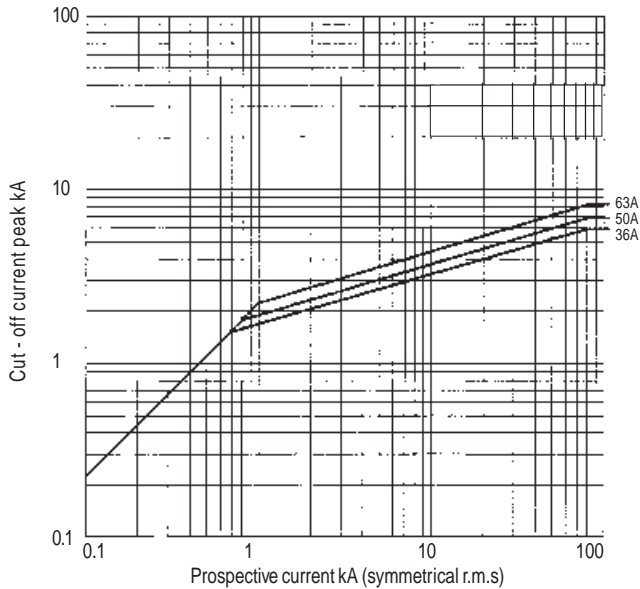
Cut-off characteristics
