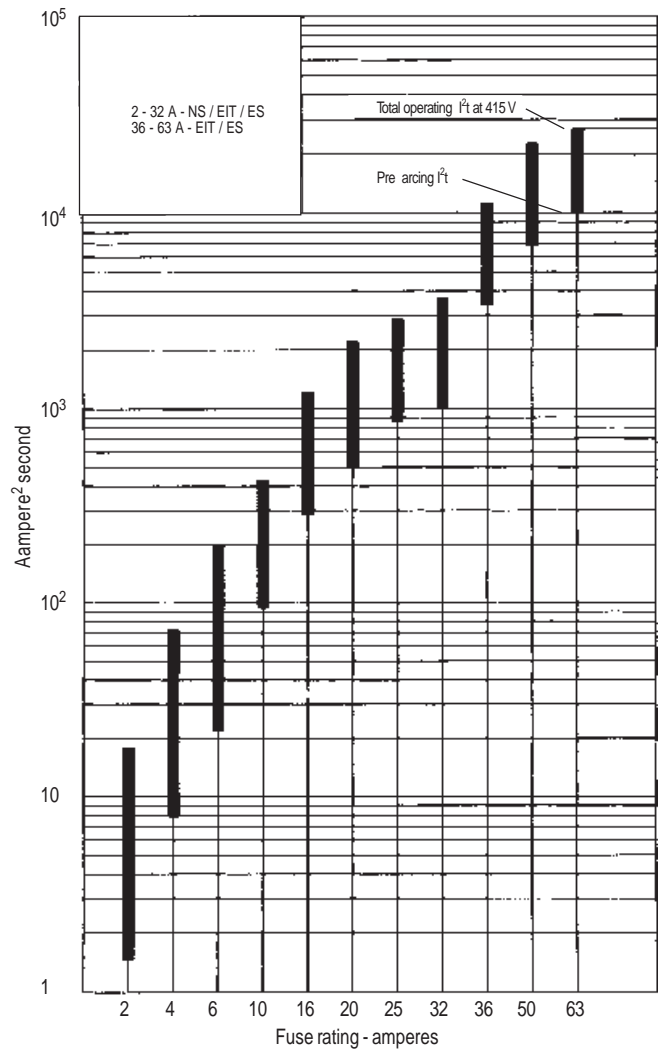
I^2t characteristics
