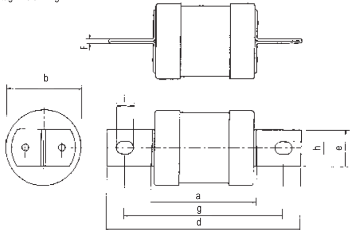
Central tag 2 hole fixing
