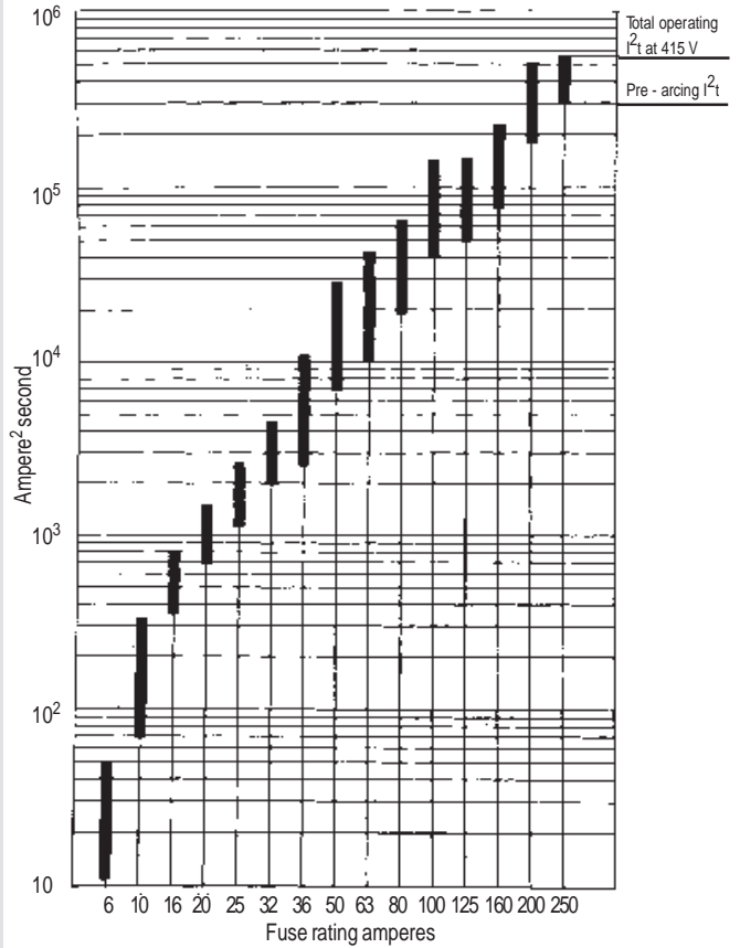
I^2t characteristics
