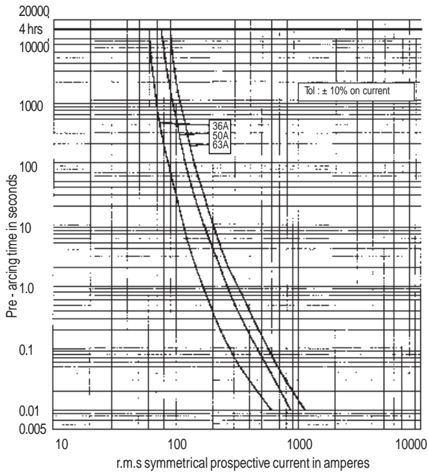
Time current characteristics
