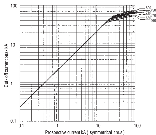
Cut - off characteristics
