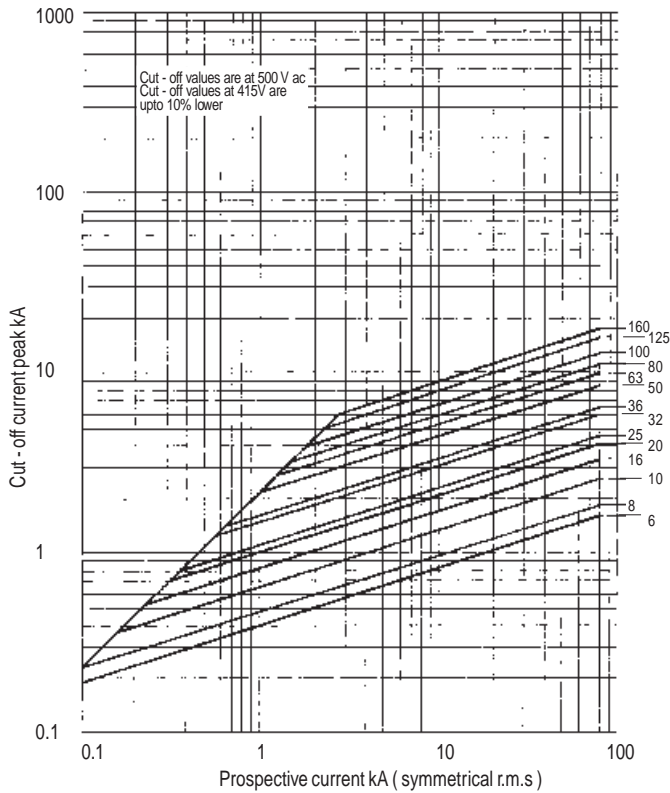
Cut - off characteristics
