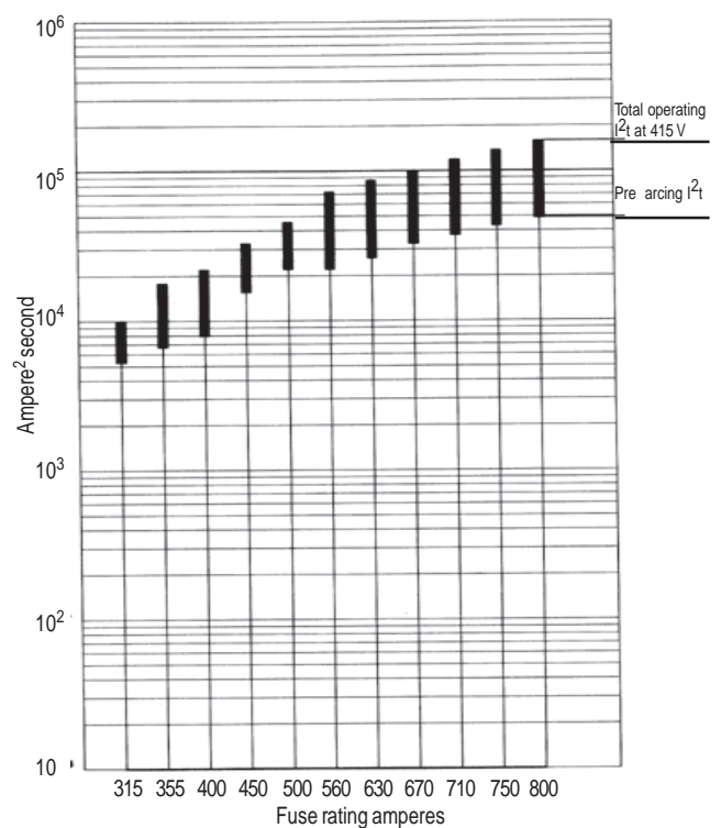
I^2t characteristics
