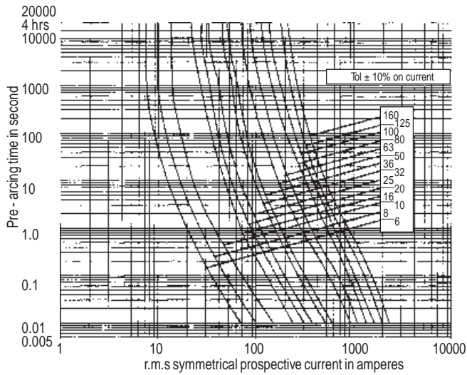
Time current characteristics
