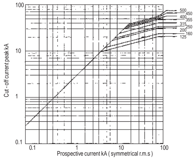
Cut - off characteristics
