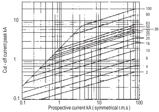
Cut - off characteristics
