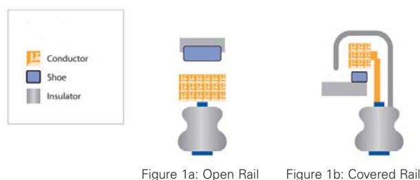
Figure 1a: Open Rail
