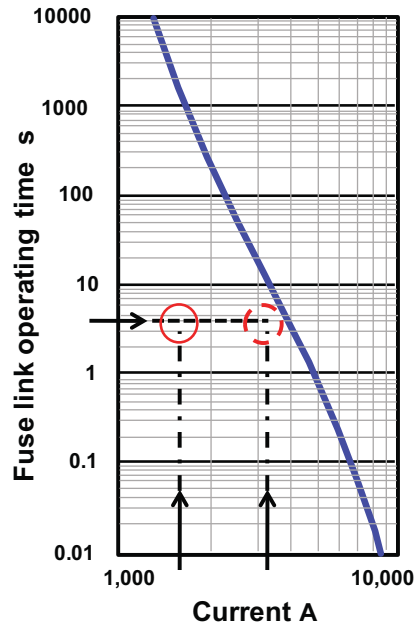
Figure 6: Time-current curve showing overload
