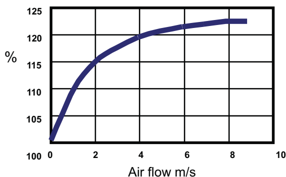
Figure 4: Improvement of current carrying capability with airflow
