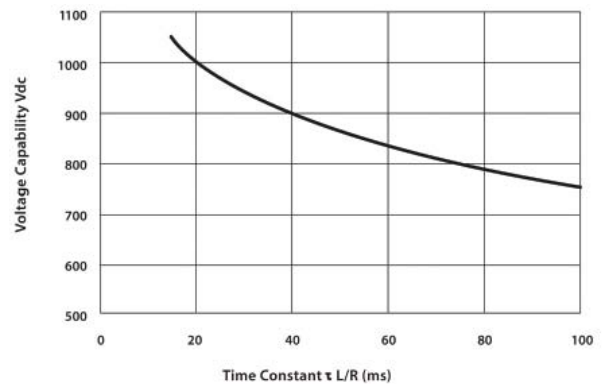
Figure 7: Voltage capability curve
