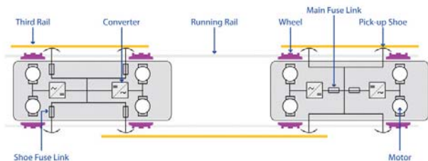
Figure 3: Fusing Options
