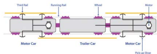
Figure 2: Typical Shoe and Power Arrangement (sub surface)
