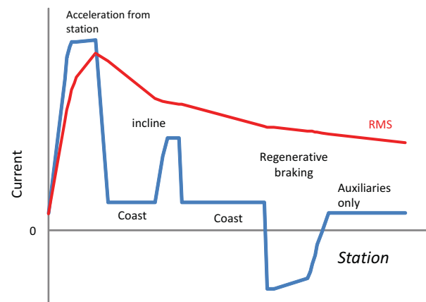
Figure 5: Typical current profile between stations
