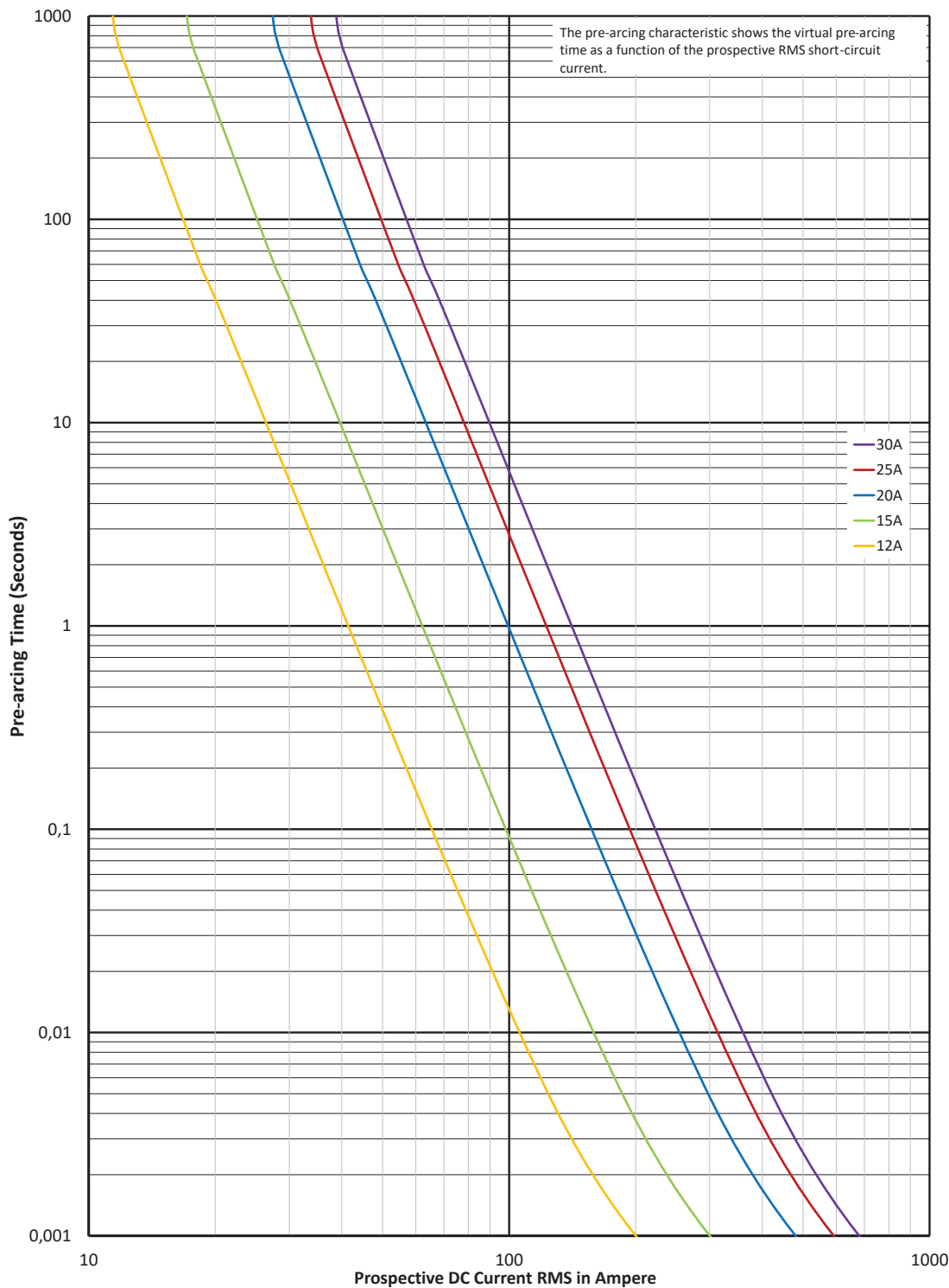
Time-current curve
