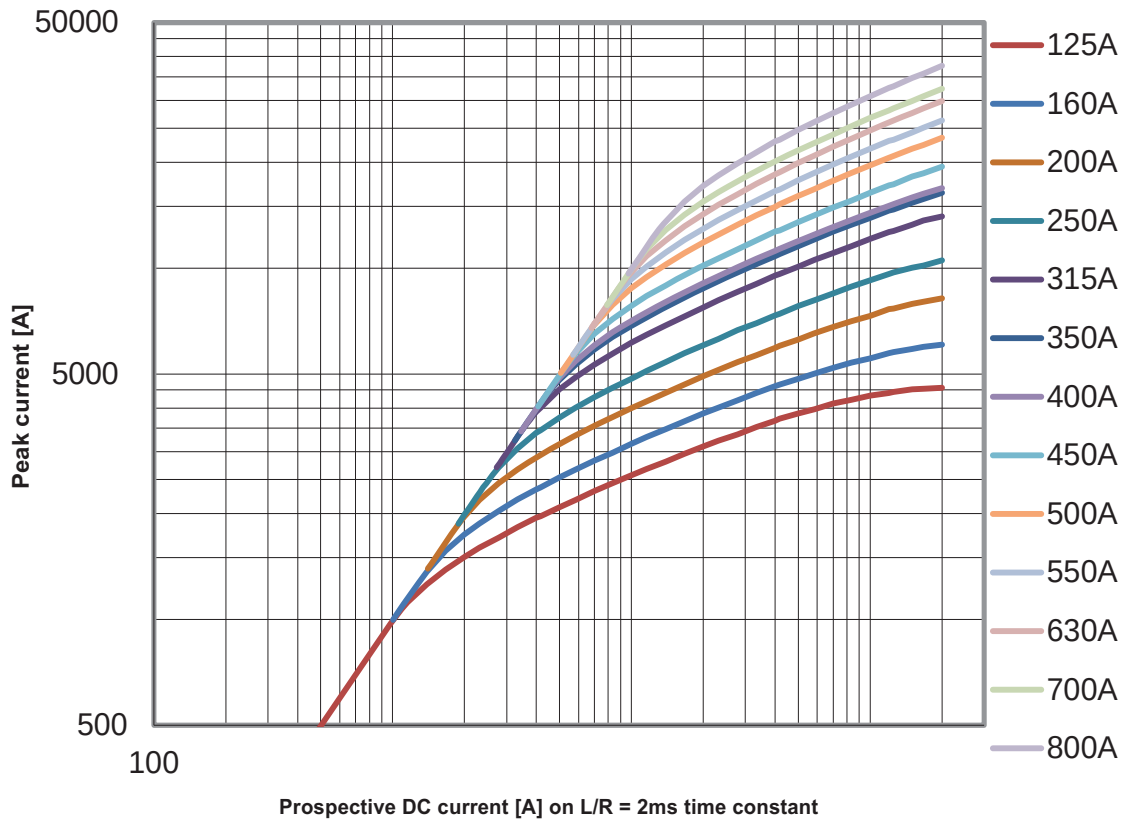
Cut-off curve
